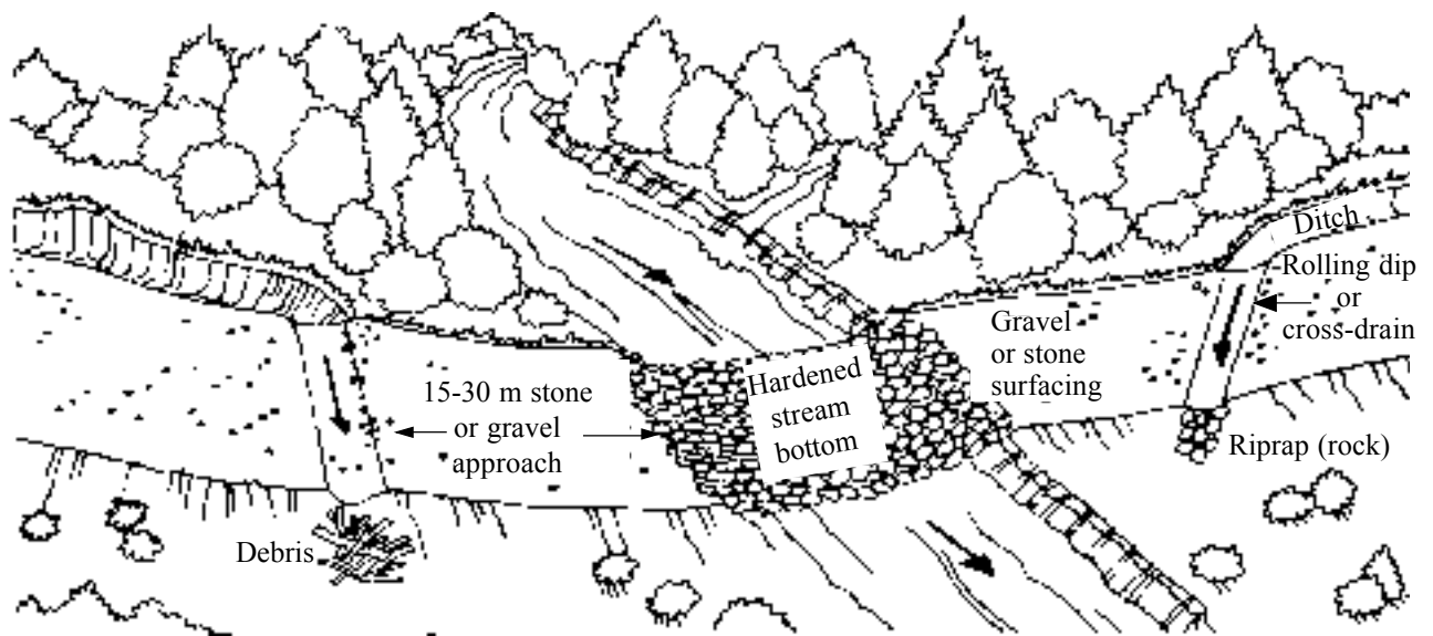
Figure 7.12 Protection measures at stream crossings.
