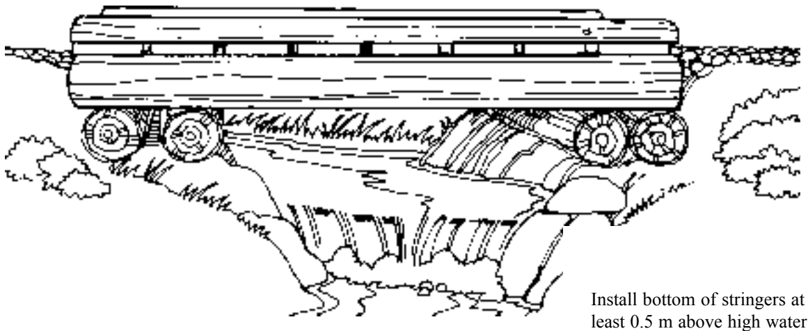
Figure 10.2 Bridge installation with simple foundation details.
